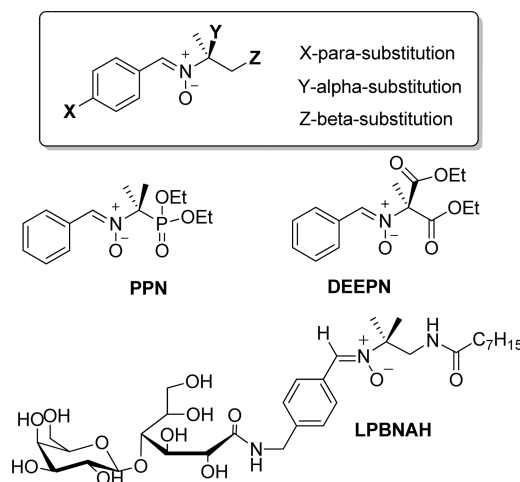
Figure 1. General structure and some examples of substituted linear nitrones.
