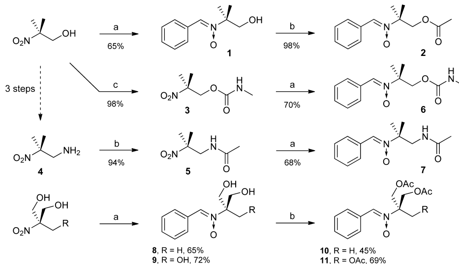
Scheme 1. Synthesis of Mono-, Di-, and Tri- \beta -Substituted Nitrones a
